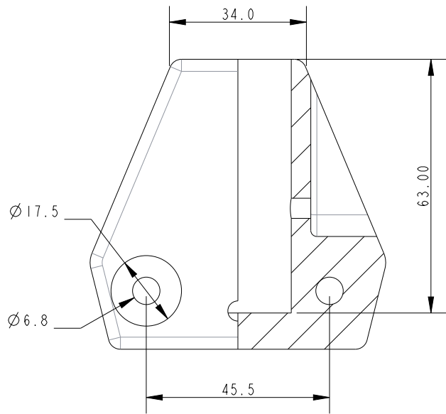
SECTION A-A SCALE 3:4
